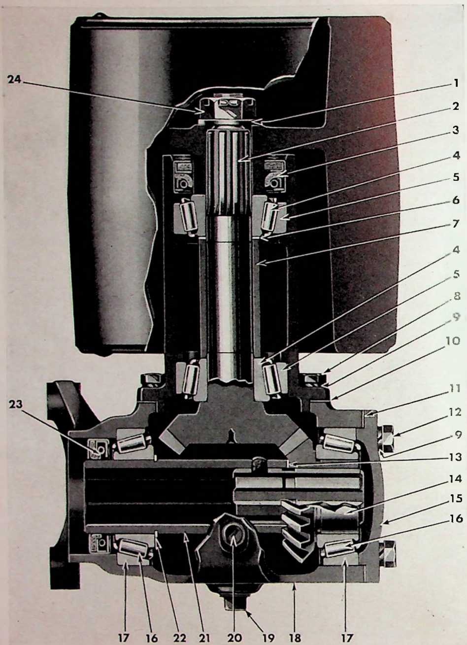
FIG. 64—PULLEY DRIVE
