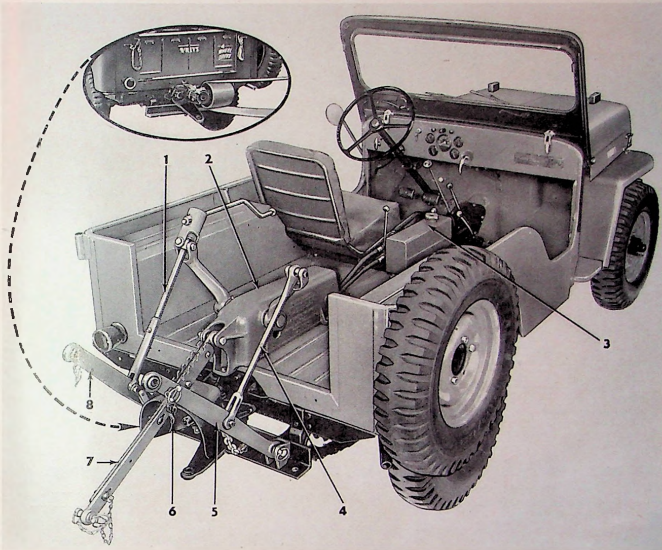
FIG. 66—HYDRAULIC LIFT
