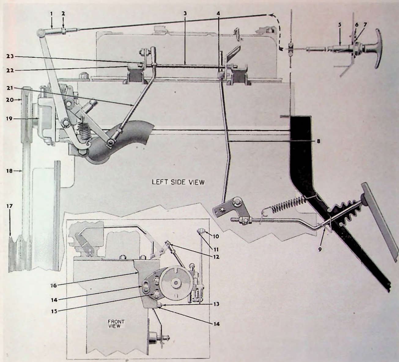
FIG. 74—GOVERNOR AND CONTROLS
