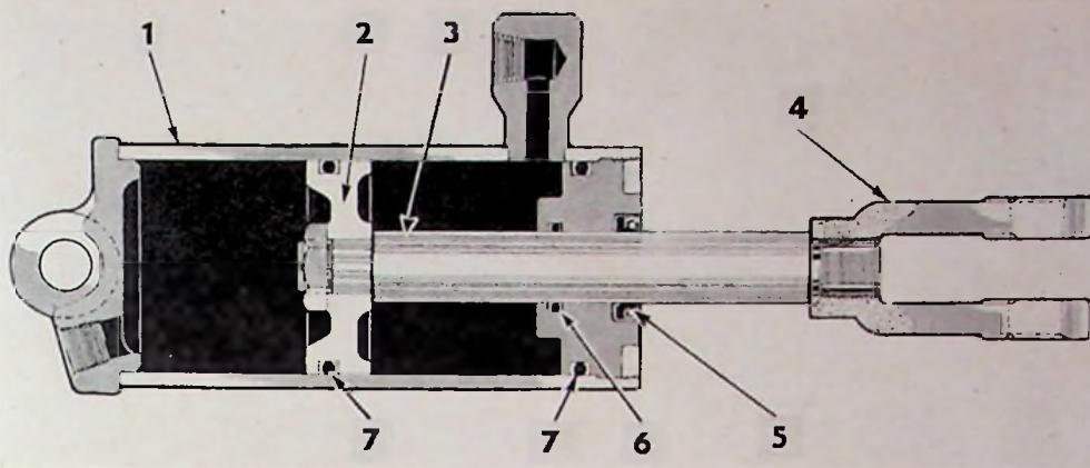
FIG. 72—HYDRAULIC CYLINDER FOR IMPLEMENT LIFT
