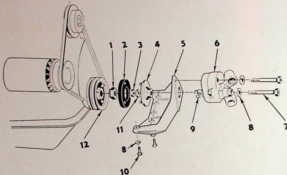
FIG. 67—PUMP AND SUPPORT FOR IMPLEMENT LIFT
