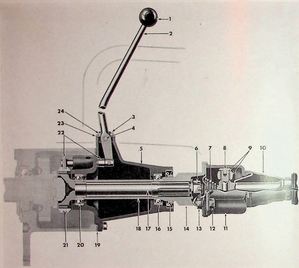
FIG. 62—POWER TAKE-OFF, FRONT UNIT
