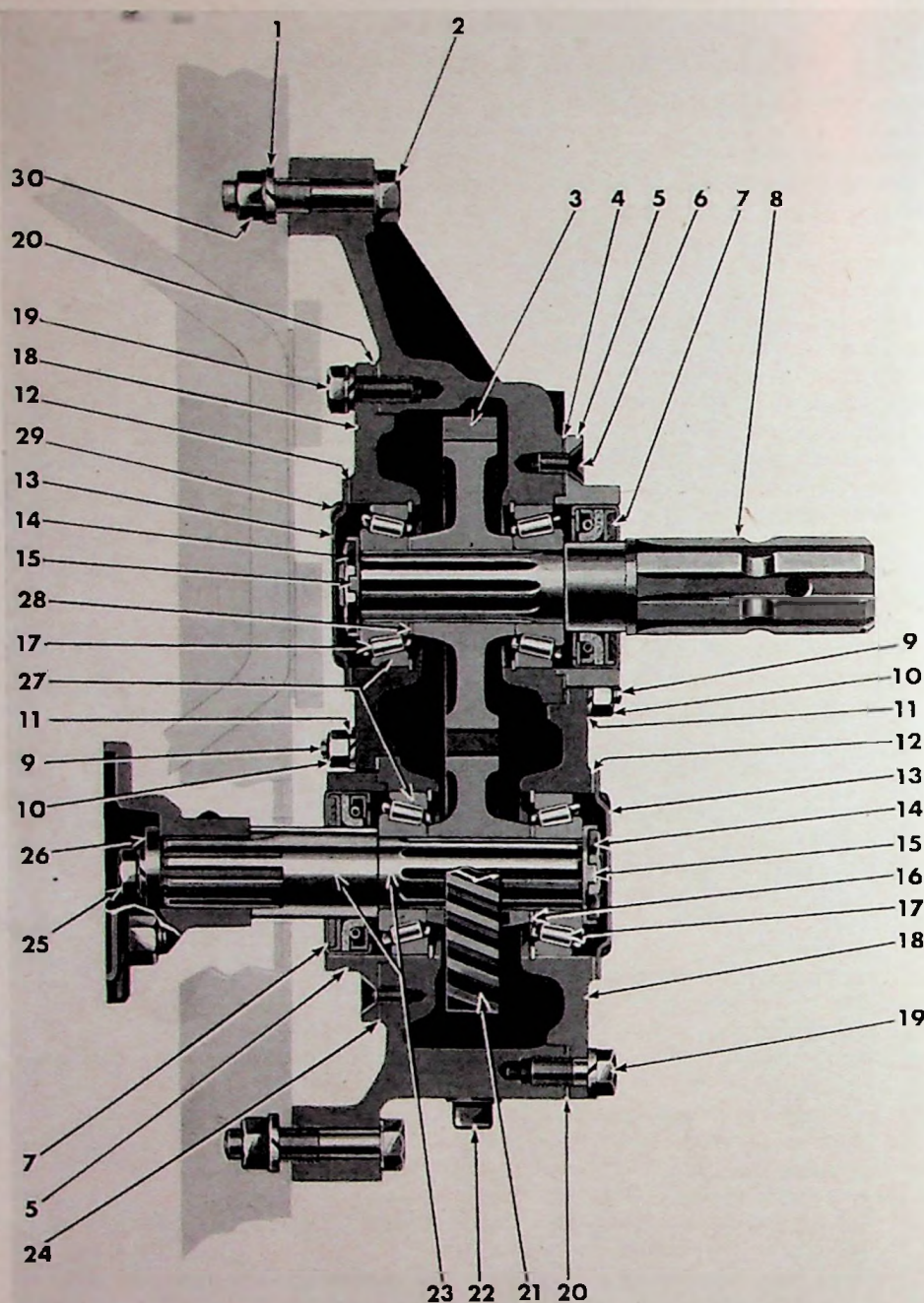
FIG. 63—POWER TAKE-OFF, REAR UNIT
