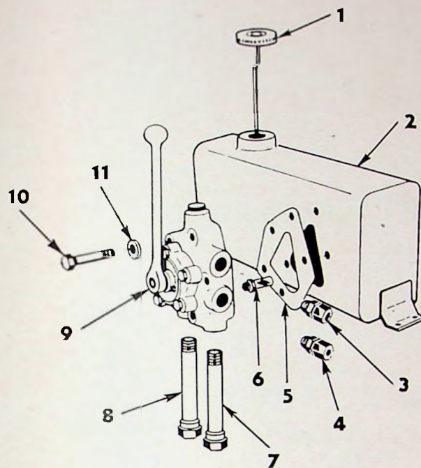
FIG. 68—TANK AND VALVE FOR IMPLEMENT LIFT
