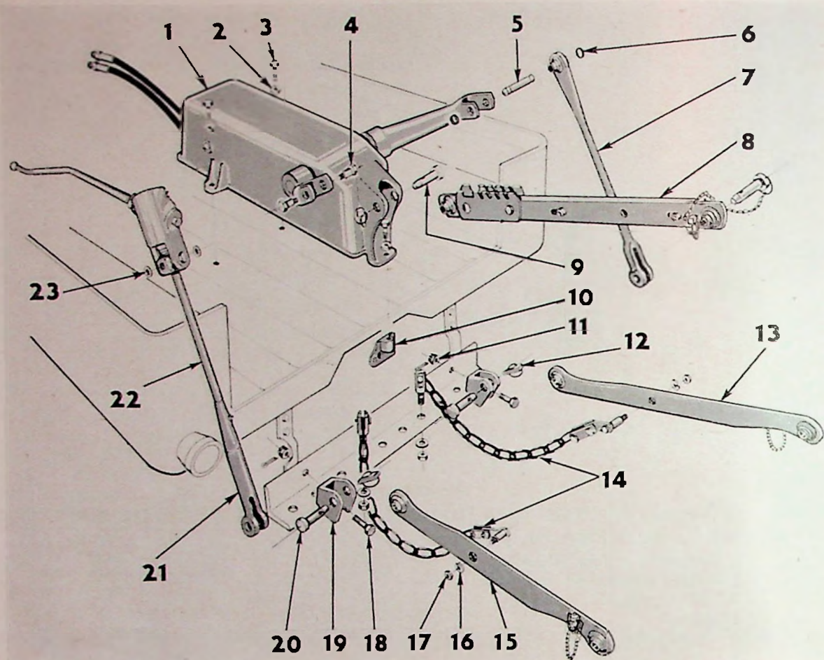
FIG. 69—MAIN HOUSING, CYLINDER AND LIFT LINKAGE
